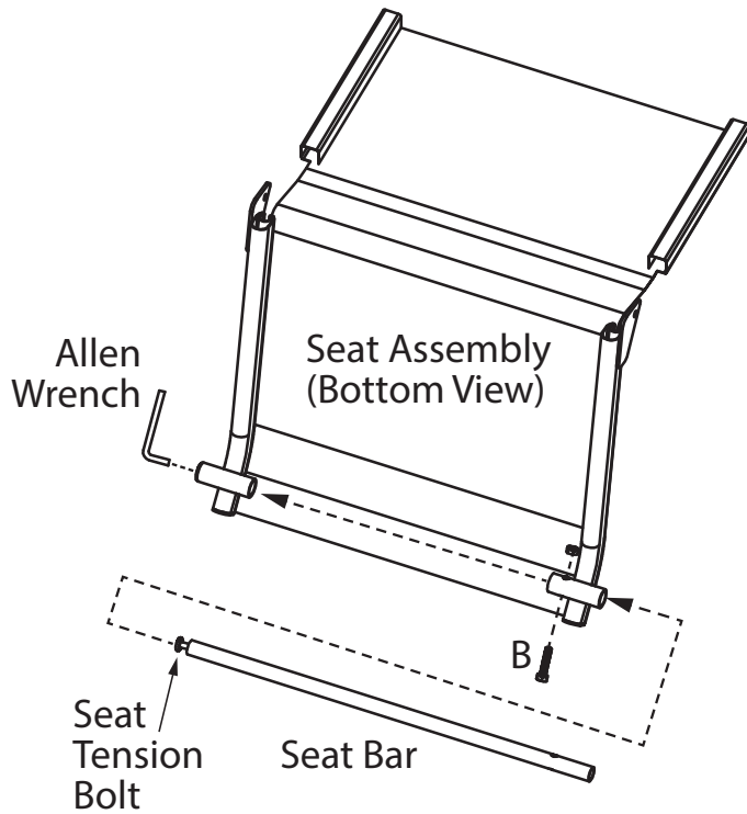
FIG 5 STEP 9. Thread the seat tension bolt completely into the seat bar . Insert the seat bar through the front of the seat assembly and secure using (1) 1/4" x 1 1/4" hex bolt [B] and (1) 1/4" nylock nut. Then, using the allen wrench turn the seat tension bolt counterclockwise until the seat is taught.
