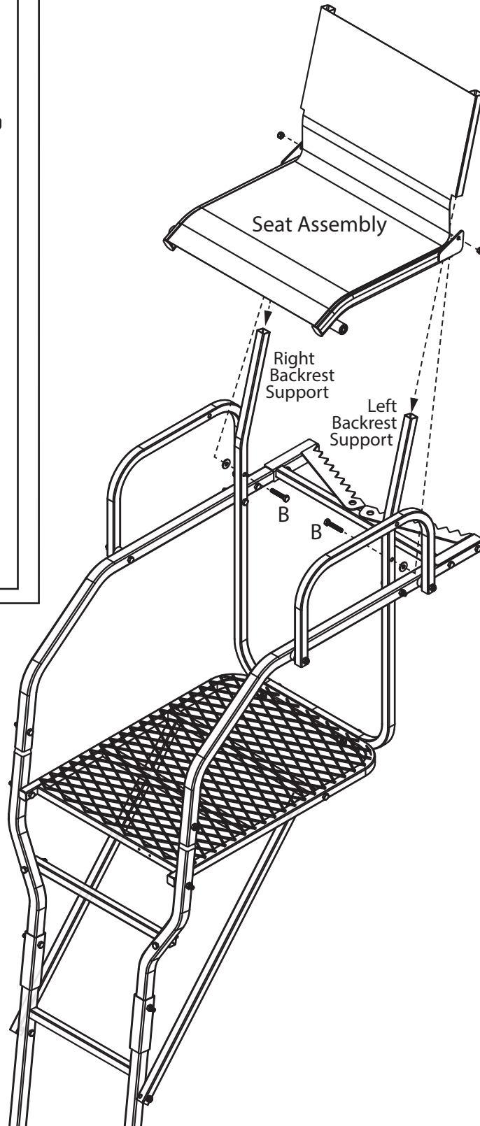
FIG 6 STEP 10. Slip the backrest of the seat assembly over the backrest support . Then, attach the seat assembly to the backrest support using (2) 1/4" x 1 1/2" hex bolts [B], (2) nylon washers and (2) 1/4" nylock nuts.
