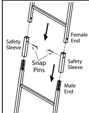
Ladderstand Install FIGURE 1A
