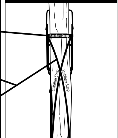
LADDERSTAND INSTALL FIGURE 5
