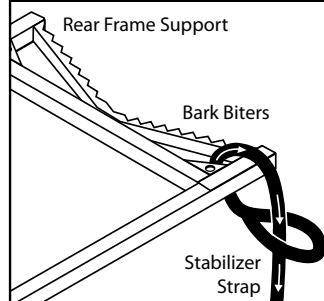
LADDERSTAND INSTALL FIGURE 2
